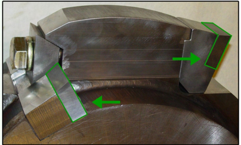
T-3 insert hammer and 1.5" x 6" tooth shown.
